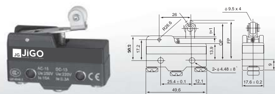
JG - XZ-15GW22-B - Micro Switch Patti Roller
