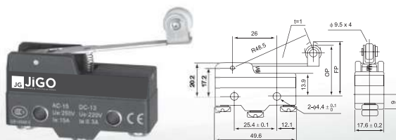
JG - XZ-15GW2-B - Micro Switch Long Patti Roller
