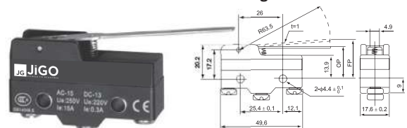
JG - XZ-15GW-B - Micro Switch Long Patti
