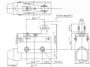
JG - XZ-7141 - Micro Switch Short Hinge Roller Lever
