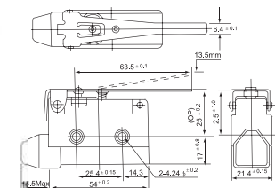
JG - XZ-7120 - Micro Switch Long Hinge Lever
