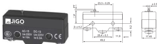
JG - XZ-15G-B - Micro Switch Dot Point
