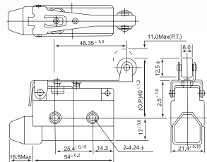
JG - XZ-7121 - Micro Switch Long Hinge Roller Lever
